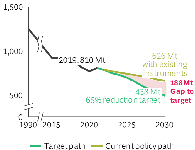
GHG 1 emissions in Germany 1990-2030 (Mt CO 2 e)
